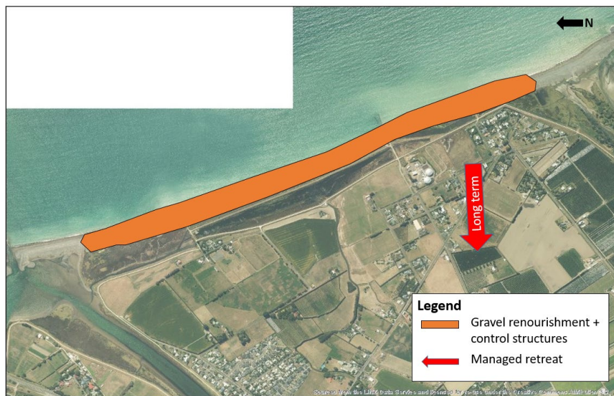
Indicative renourishment and groynes, and retreat the line/managed retreat location at East Clive.
